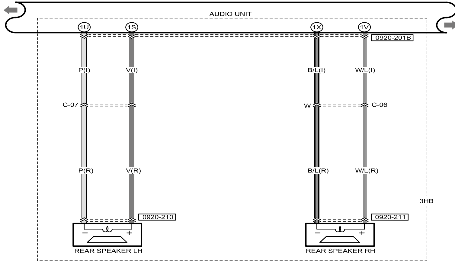
0920-210 REAR SPEAKER LH
