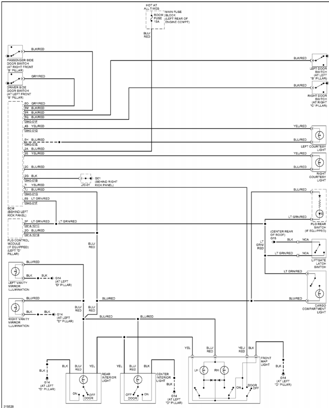
Fig. 30: Courtesy Lamps Circuit
